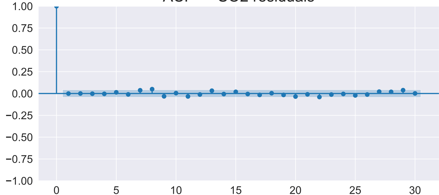
ACF — SO2 residuals
